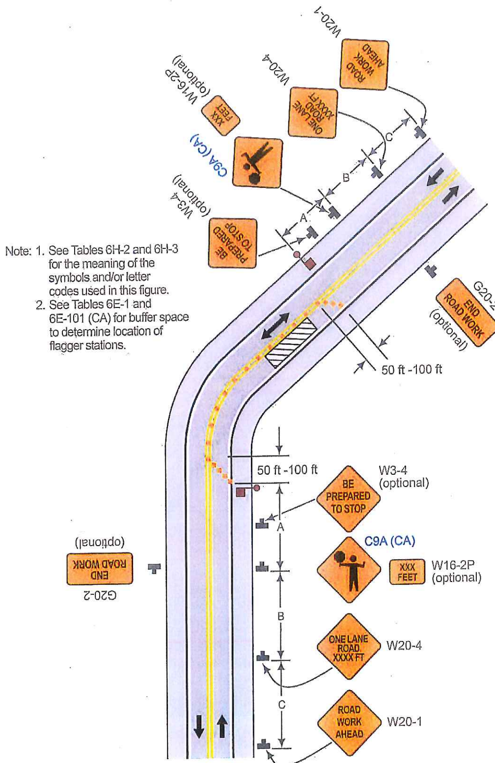
Typical Application 10
